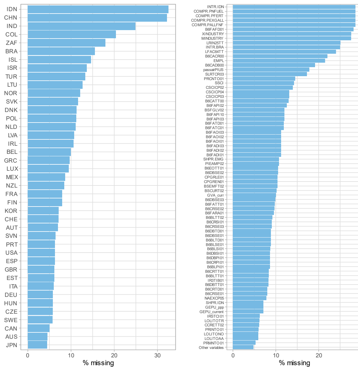
Figure A.1. Percentage of missing values
